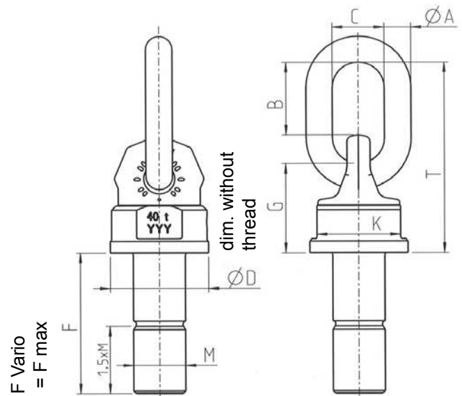
Pic. 6: Dimensioning VWBG
