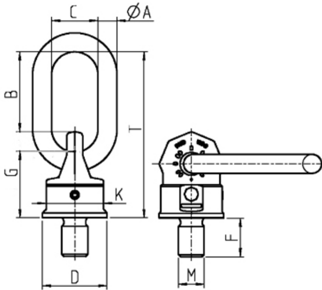
Pic. 5: Dimensioning VWBG (metric)
