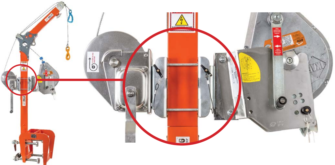
Typical application
