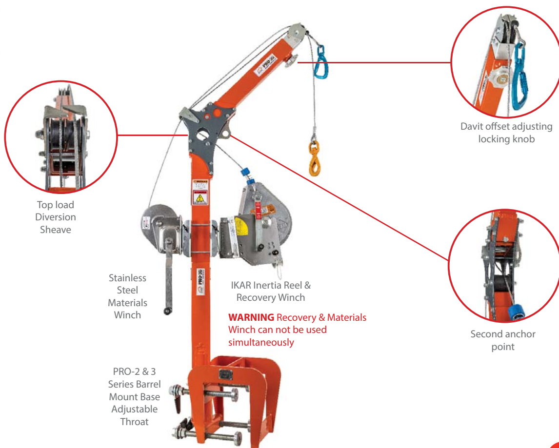
Typical Set-up
